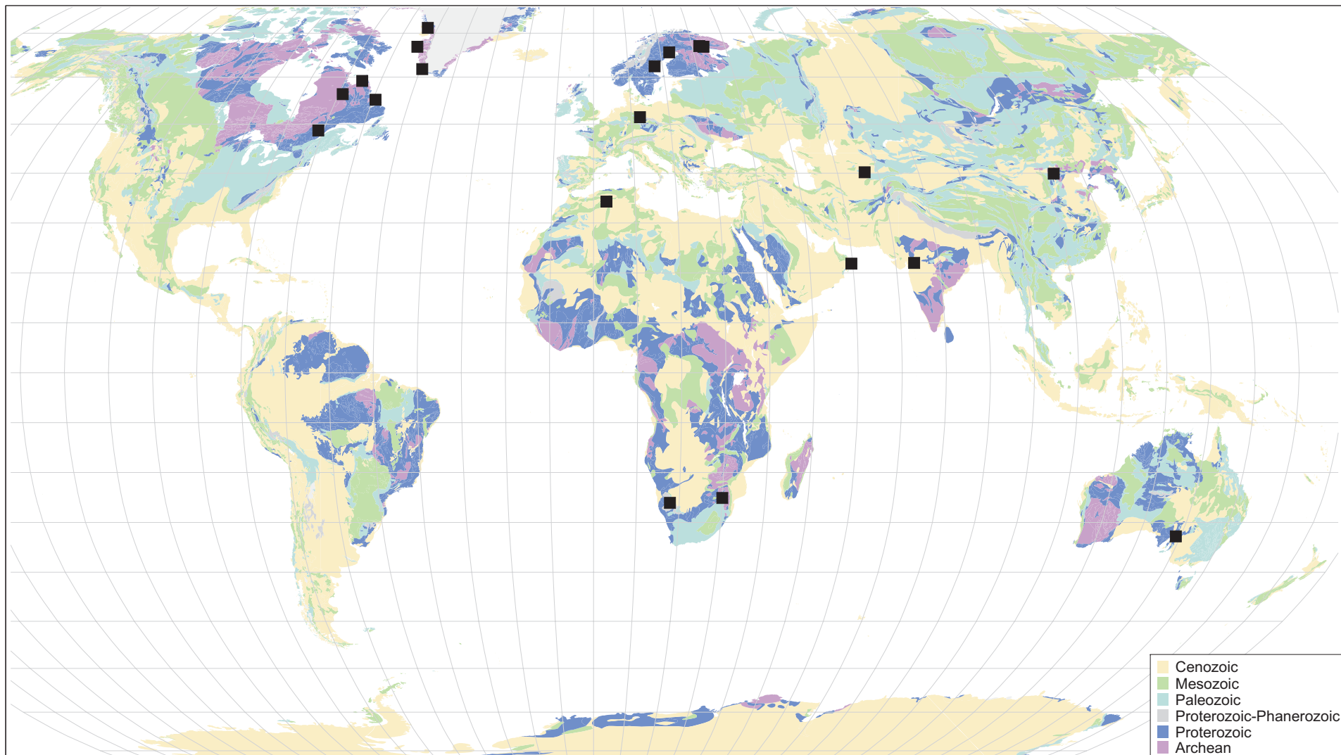
Figure 9. Localities of occurrences with lamprophyre - carbonatite association.
