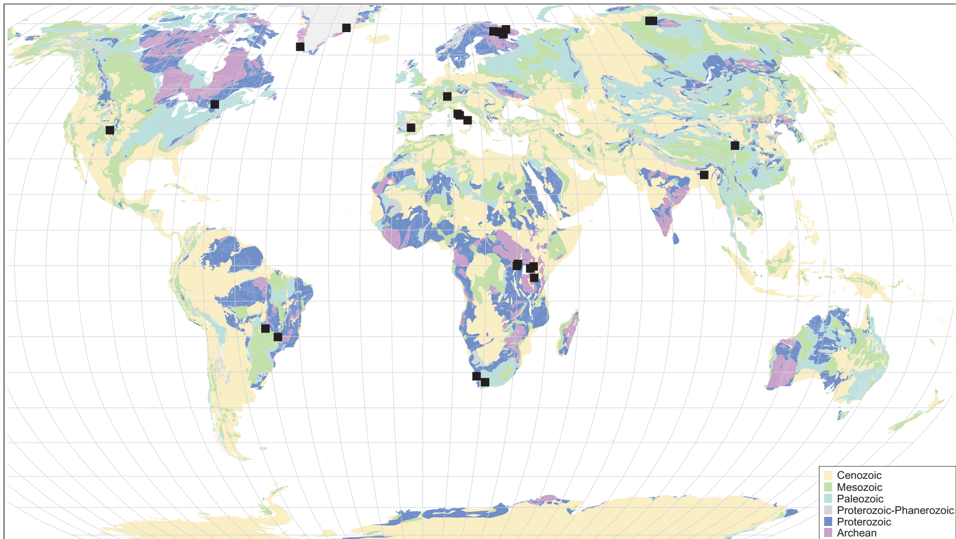
Figure 3. Localities of occurrences with melilitite (melillolite) - carbonatite association.
