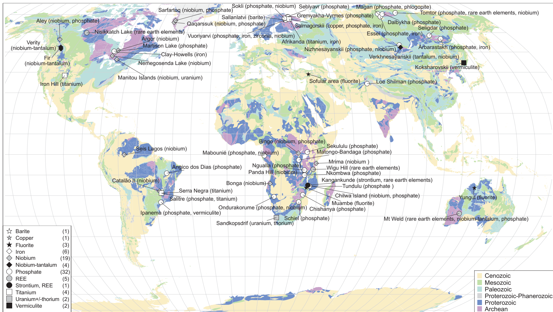
Figure 22. Carbonatite localities of economic interest that are deposits, subdivided by commodity type.
