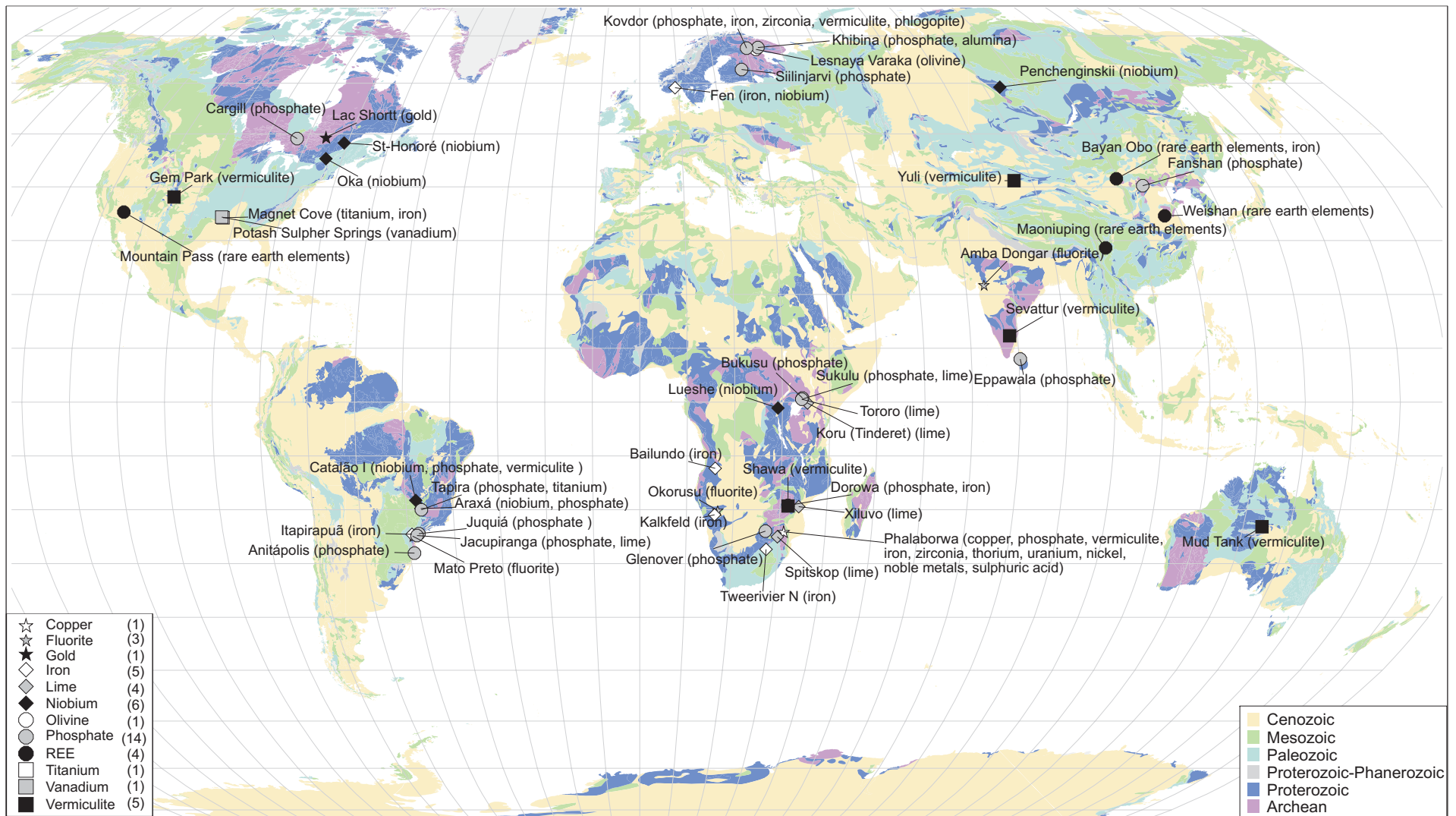
Figure 21. Carbonatite localities of economic interest that are active mines or past producers, subdivided by commodity type.
