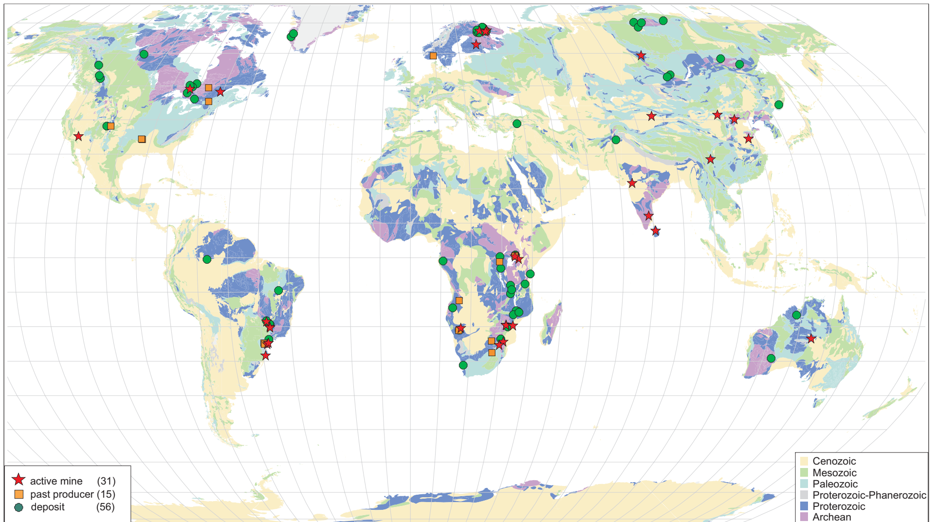
Figure 20. Carbonatite localities of economic interest, subdivided by active mine, past producer, and deposit.
