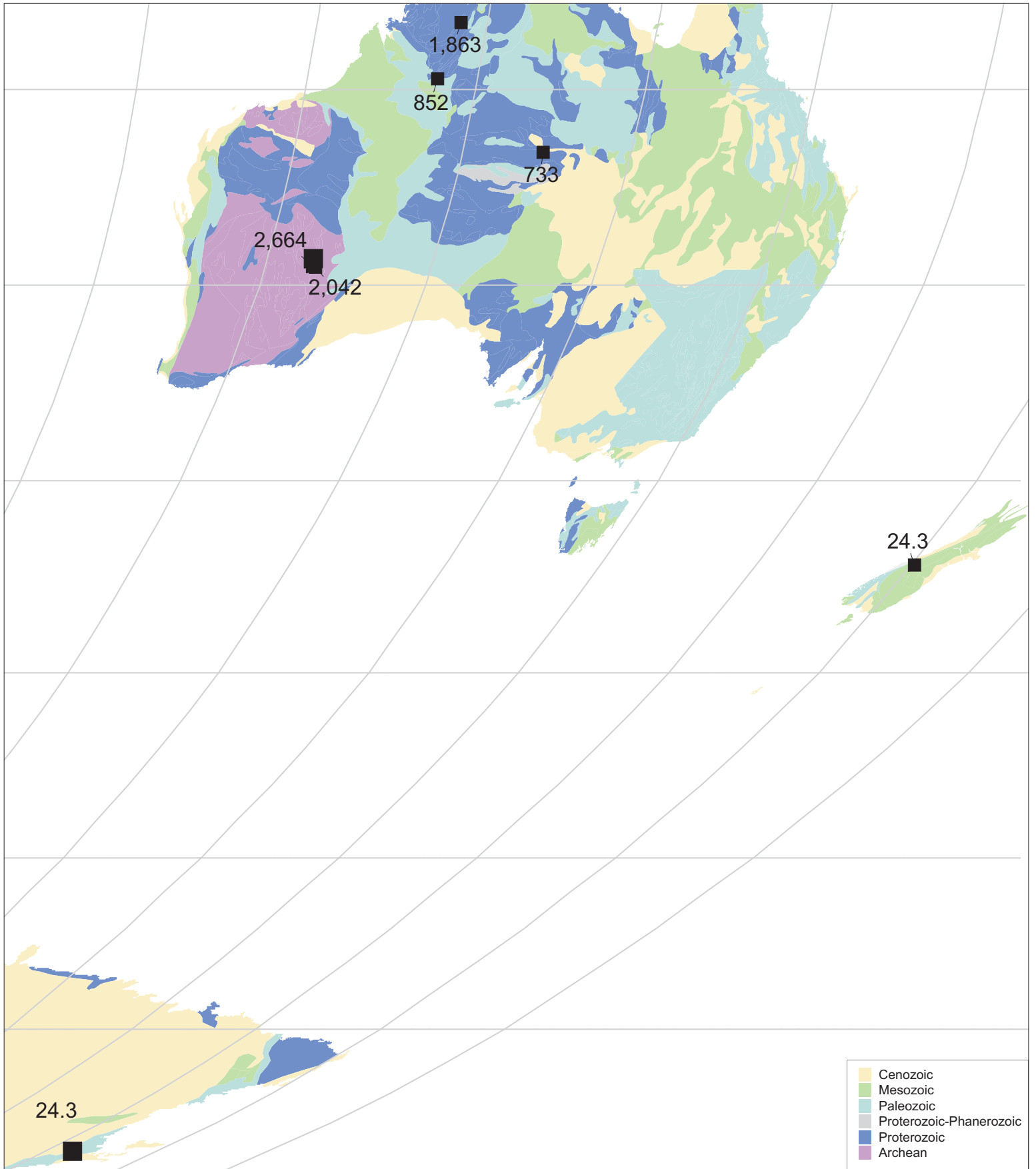
Figure 17. Ages of carbonatite occurrences in Australasia and Antarctica.
