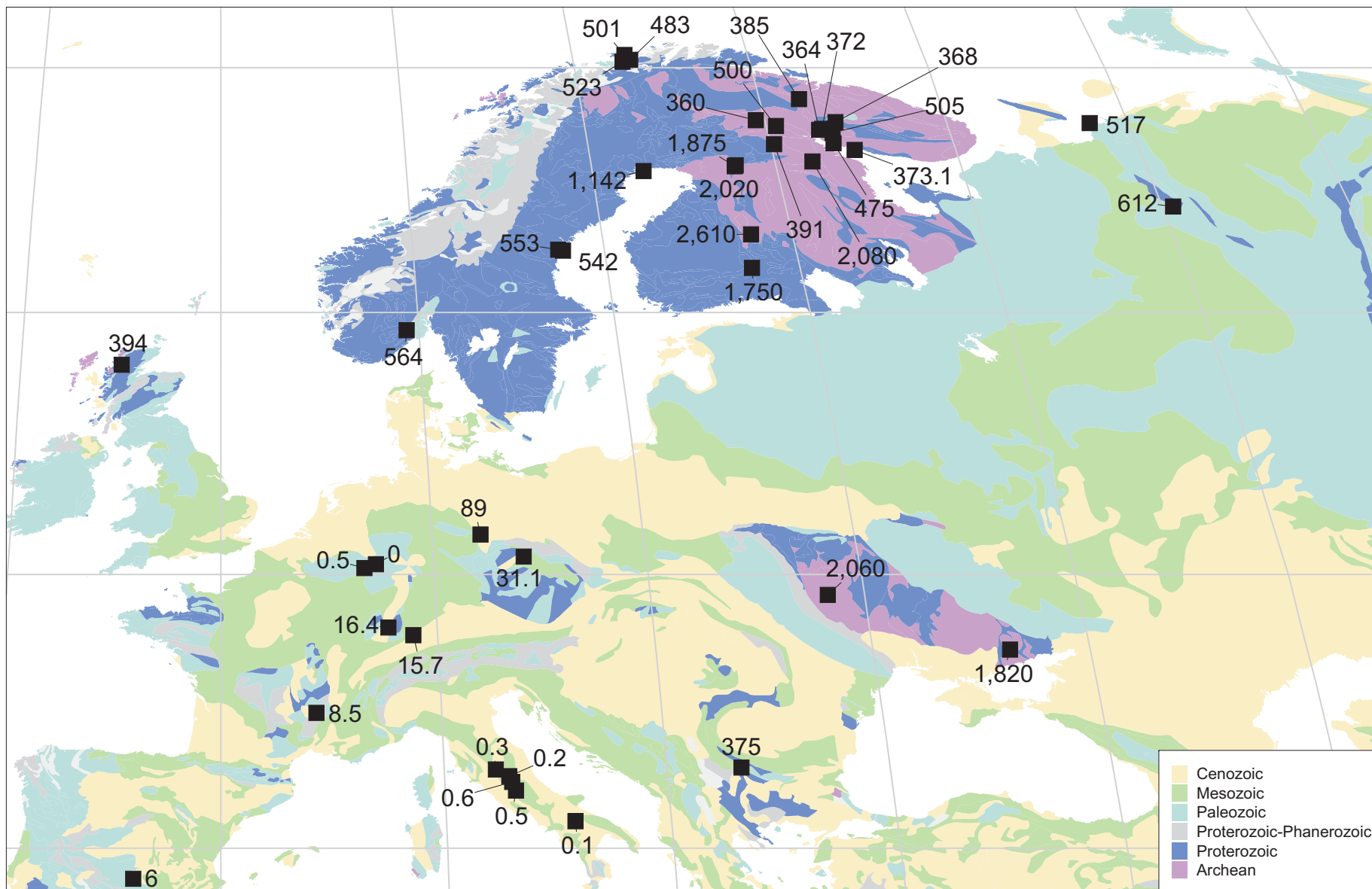
Figure 16. Ages of carbonatite occurrences in Europe and Russia west of the Ural Mountains.
