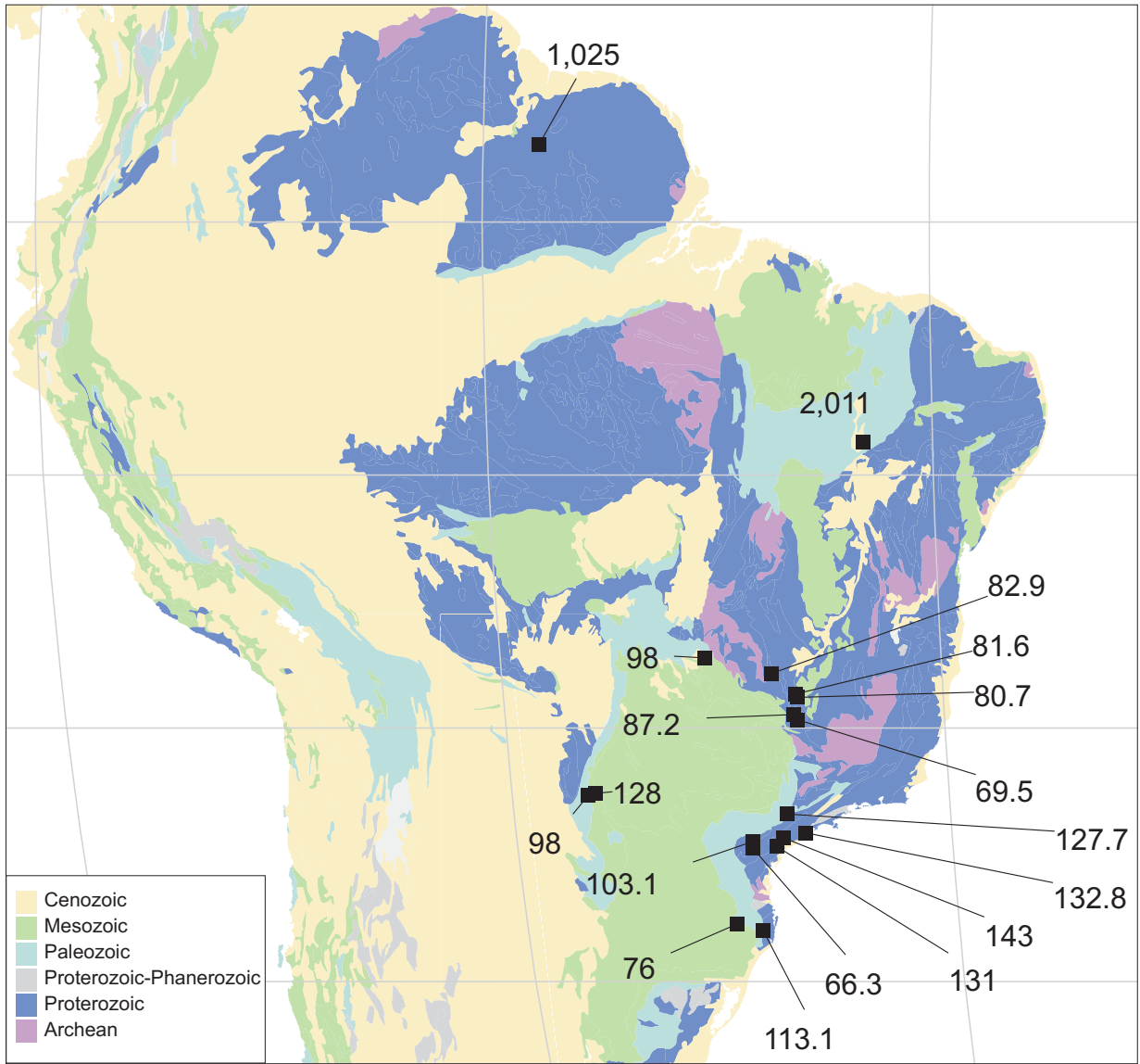
Figure 15. Ages of carbonatite occurrences in South America.
