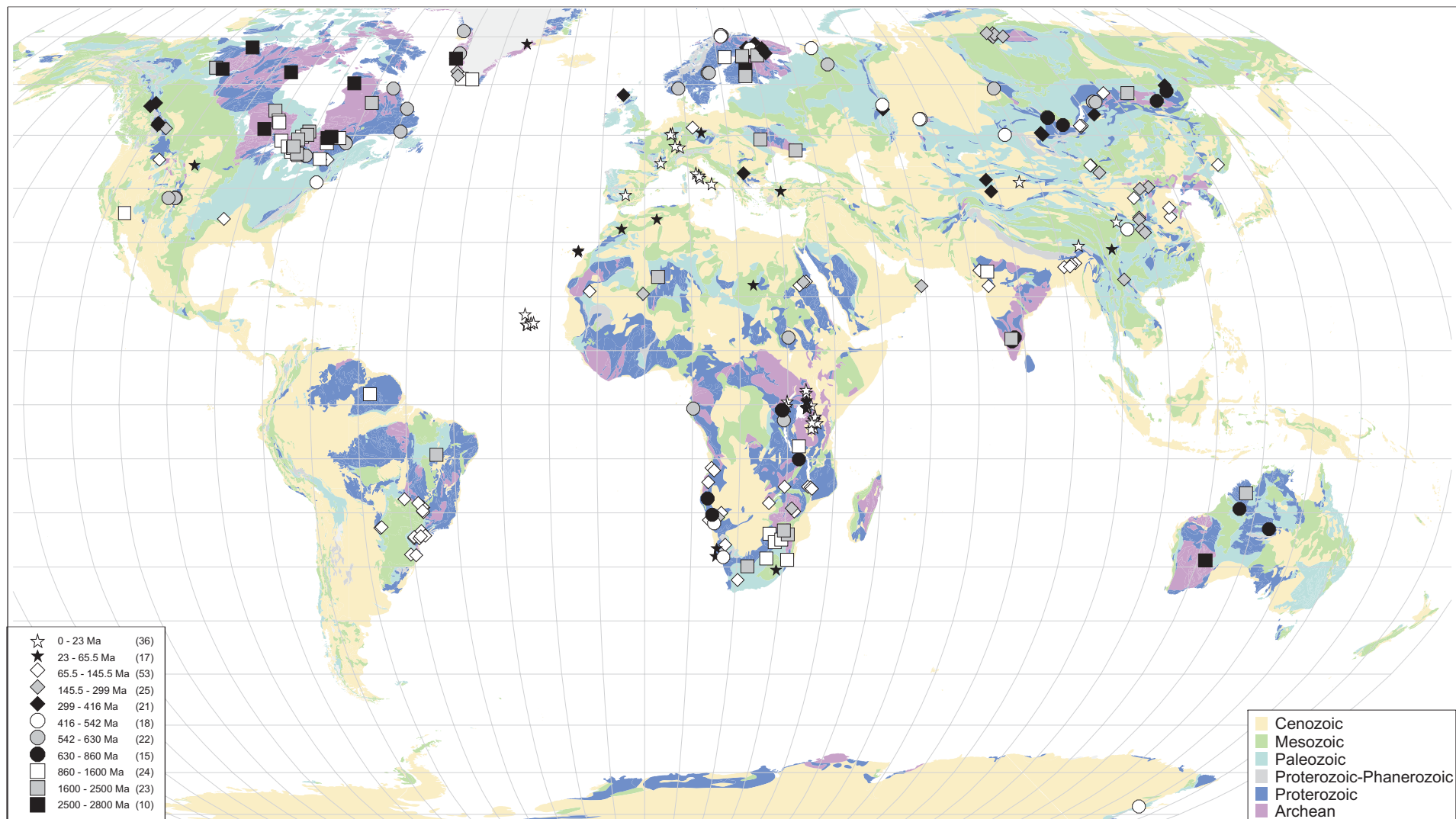
Figure 13. Carbonatite ages plotted on the world map and subdivided into eleven age groupings.
