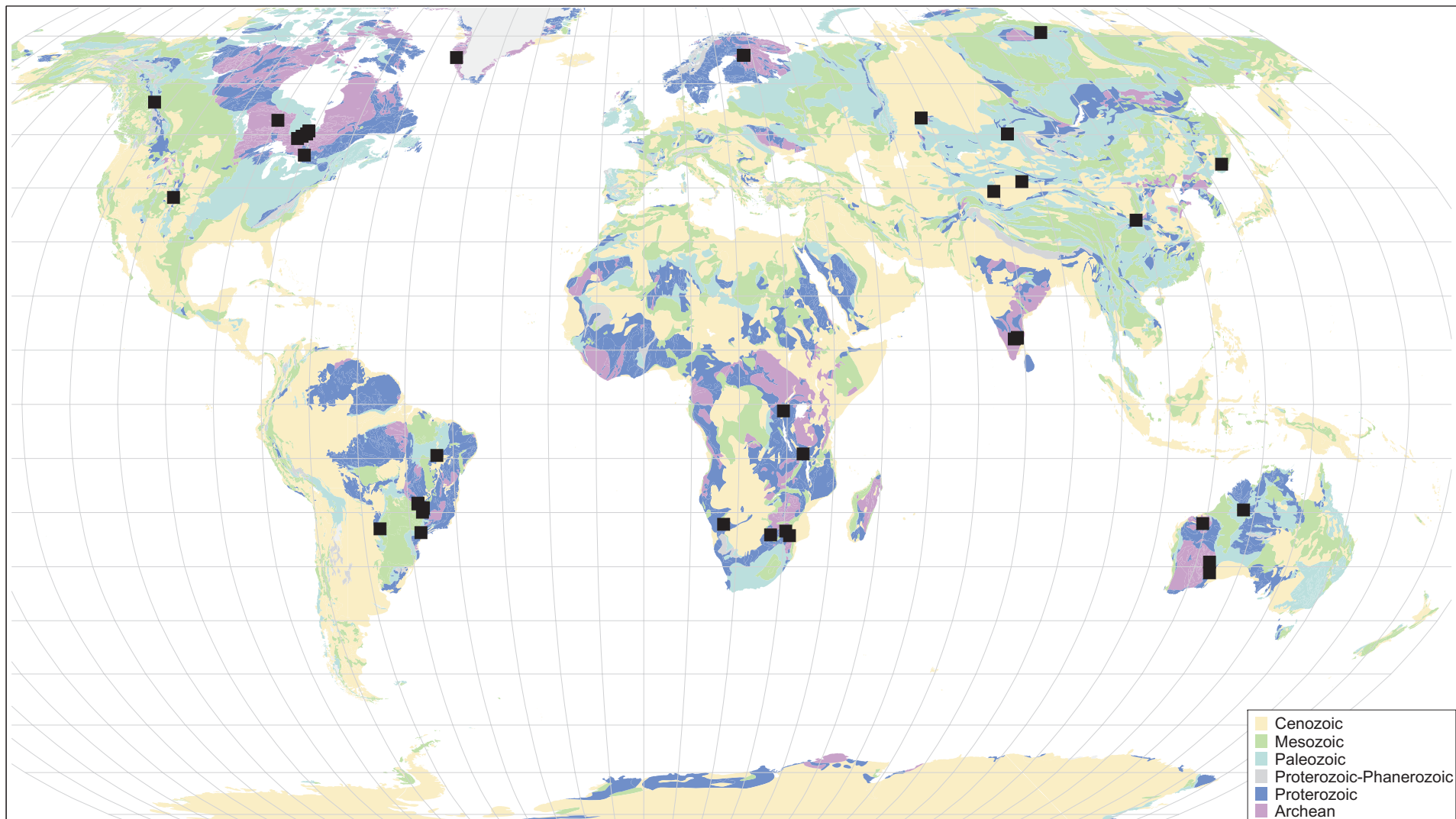
Figure 11. Localities of occurrences with carbonatite plus cumulates.
