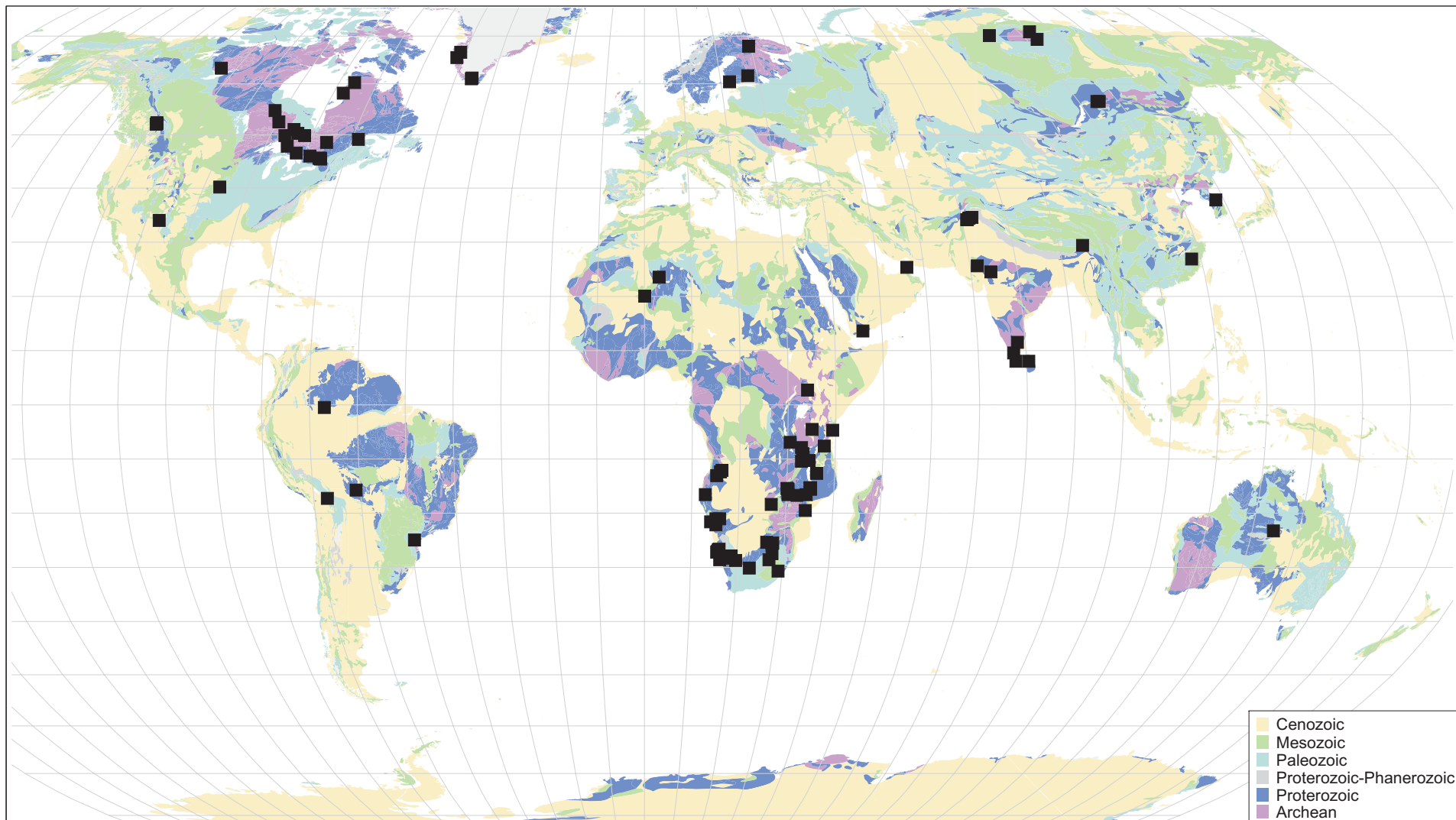
Figure 10. Carbonatite only localities.
